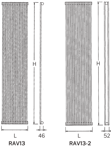
Ravenna 13 Tube diameter 13mm
